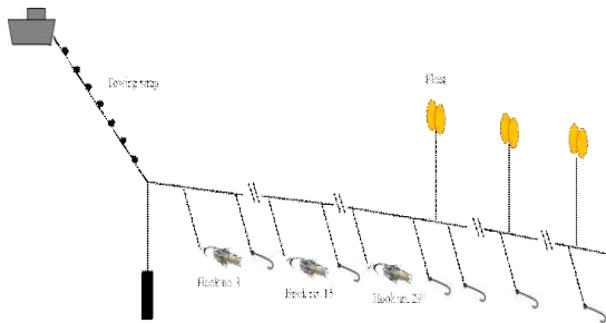
[Fig. 4] Diagram showing the installation position of underwater LED fishing light in the hairtail trolling line
